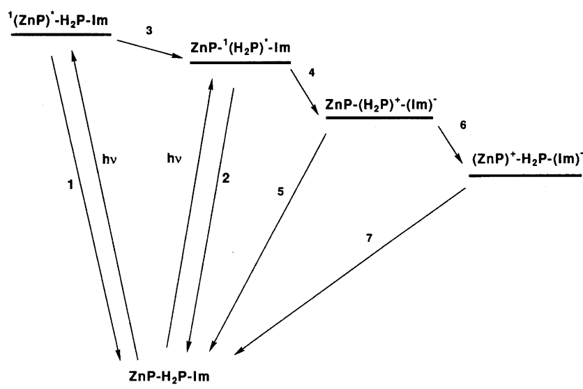
Scheme 1. Reaction scheme for triads 1a (Im=PIm) and 2a (Im=NIm). Energy levels are as follows; ^1(\text{ZnP})^* , 2.13 eV; ^1(\text{H}_2\text{P})^* , 1.97 eV; \text{ZnP-(H}_2\text{P})^+-(\text{PIm})^- , 2.00 eV; \text{ZnP-(H}_2\text{P})^+-(\text{NIm})^- , 1.64 eV; (\text{ZnP})^+-\text{H}_2\text{P-(PIm)}^- , 1.72 eV; (\text{ZnP})^+-\text{H}_2\text{P-(NIm)}^- , 1.48 eV. Energy levels of the ion pair states were calculated on the basis of the redox potentials of the chromophores measured in DMF and work terms due to static Columbic stabilization energy between the charged states.
